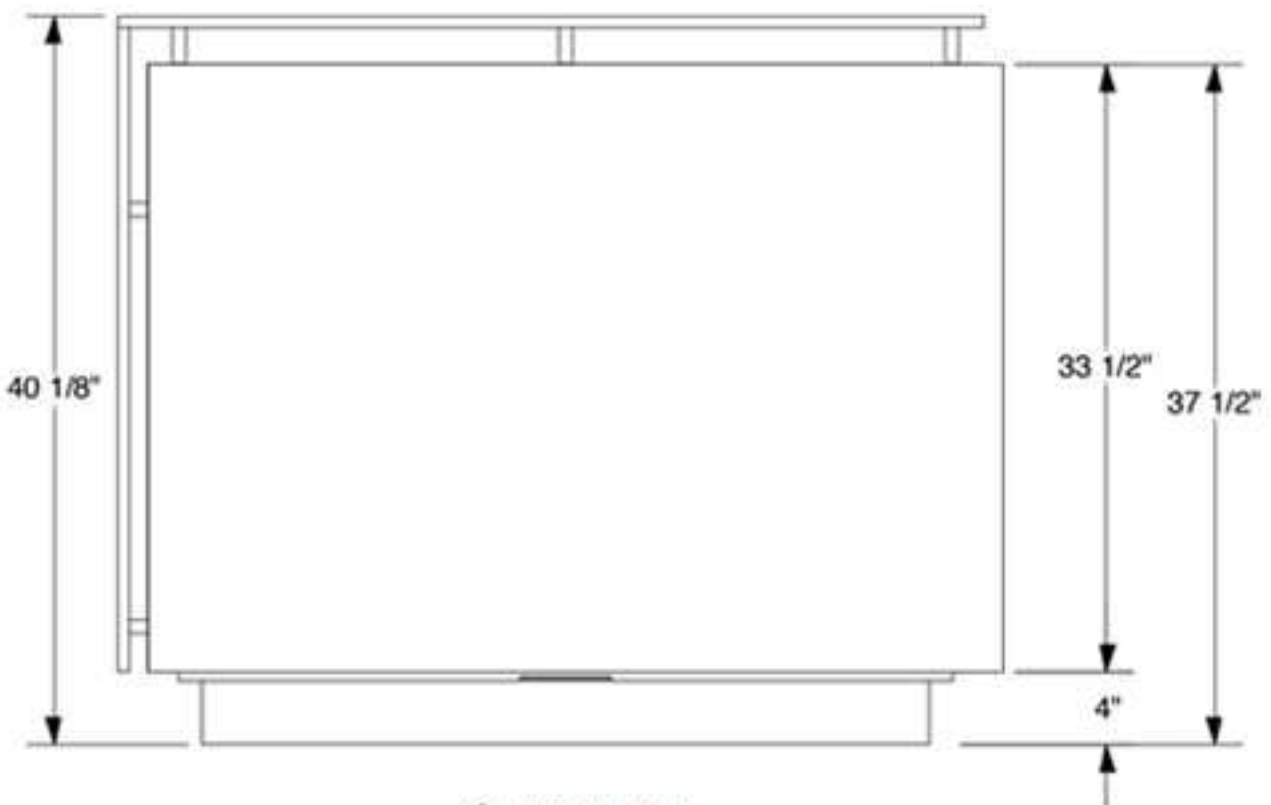
FRONT VIEW
