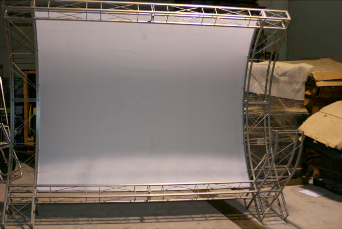
Step 5. Work your way across the bottom beam using 5 or 6 clips until the bottom of the banner is well secured.
