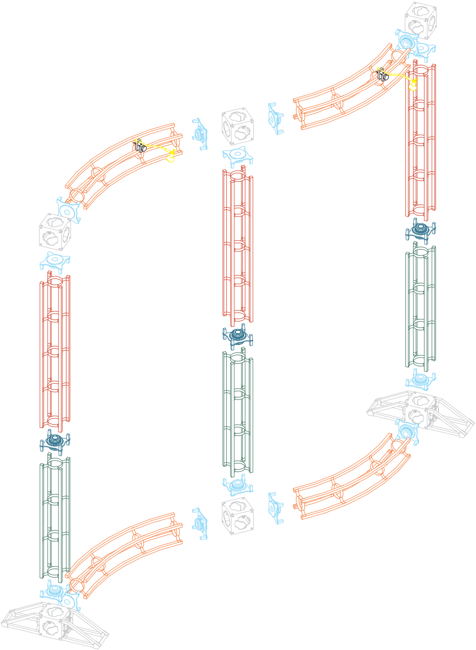
Parts exploded
