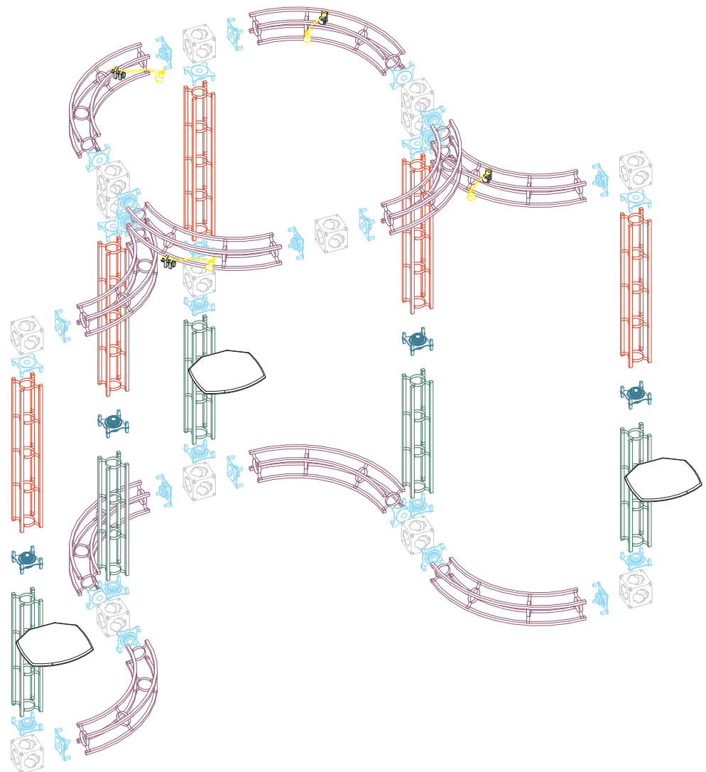
Parts exploded
